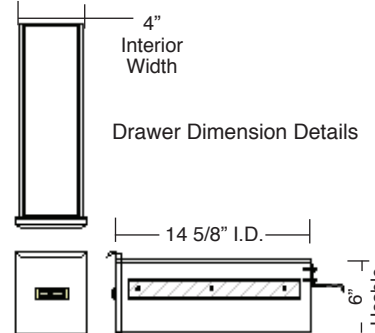
Right Side Cut-Away View
